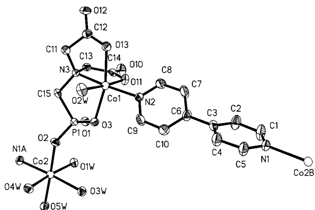
Figure 4. An ORTEP representation of the asymmetric unit of 2 ; thermal ellipsoids are drawn at the 30% probability level
