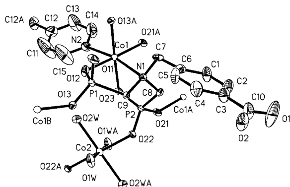
Figure 1. ORTEP representation of the asymmetric unit of compound 1 ; thermal ellipsoids are drawn at the 50% probability level
