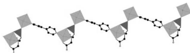
Figure 5. A 1D zigzag chain along the diagonal axis b and the -c axis in 2 ; the \text{CPO}_3 tetrahedra and \text{CoN}_2\text{O}_4 octahedra are represented by medium and light gray, respectively
